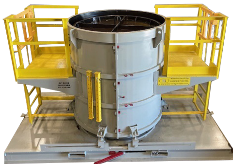
Large Diameter Quick Strip Roll Back Pipe Form
