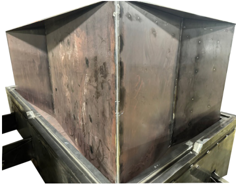
Hinged Hydraulic Collapsible Core
