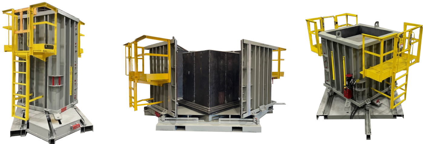
Two Piece Roll Back Form
