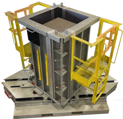
Two Piece Roll Back with Adjustable Wall Thickness
